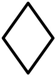
diamond
